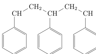
Figure 1: Polystyrene.
